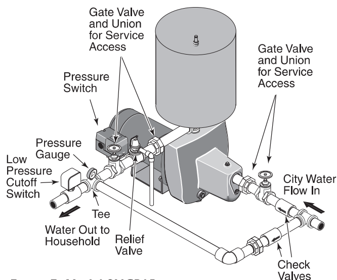
Figure 7: Model SNCP15
