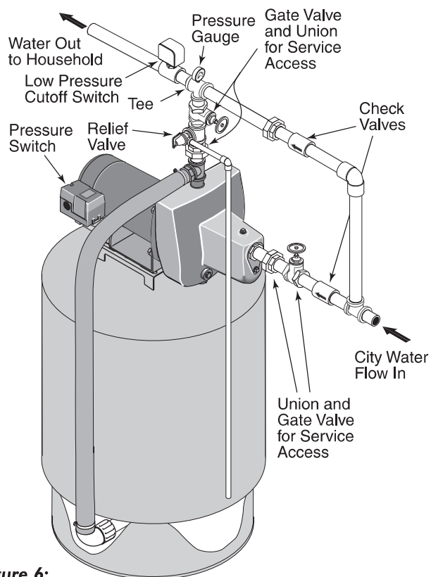
Figure 6: Model SNCP42
